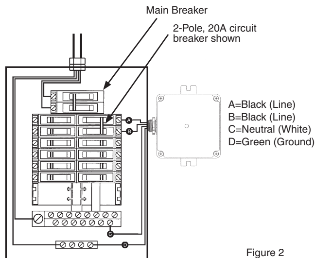
Figure 2 Type 2 Installation
